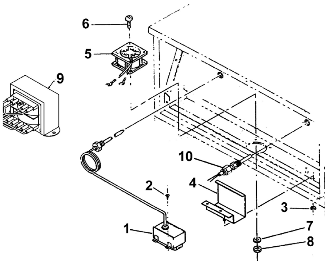
Figure 5-3. Computron 8000 - 600 – Gas Components
