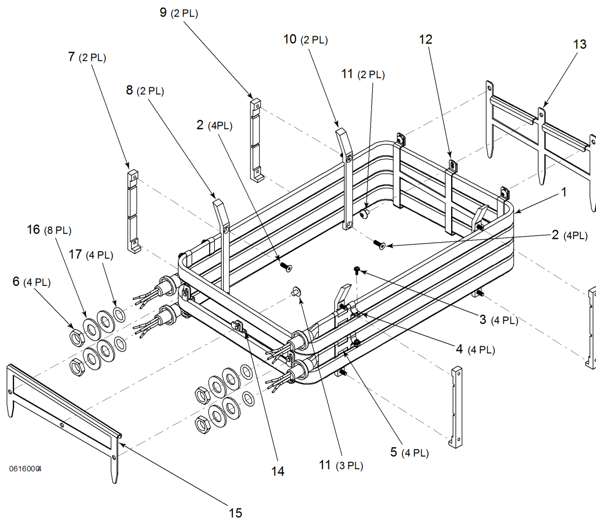
Figure 6-19 Heating Element Assy
