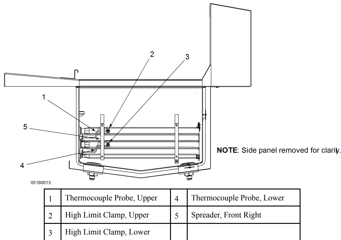
Figure 4-10 Thermocouple Installation, Right Side
