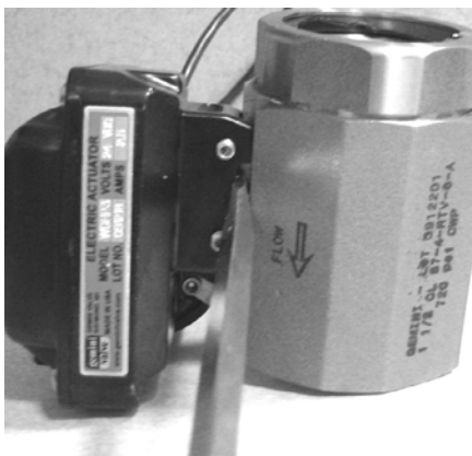
Set Screws
