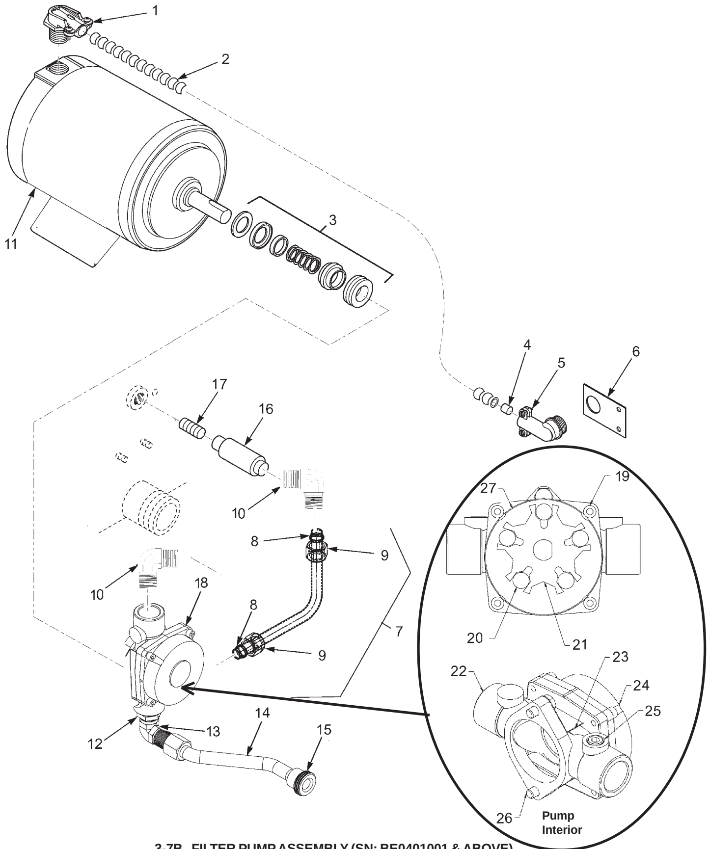
3-7B. FILTER PUMP ASSEMBLY (SN: BE0401001 & ABOVE)
