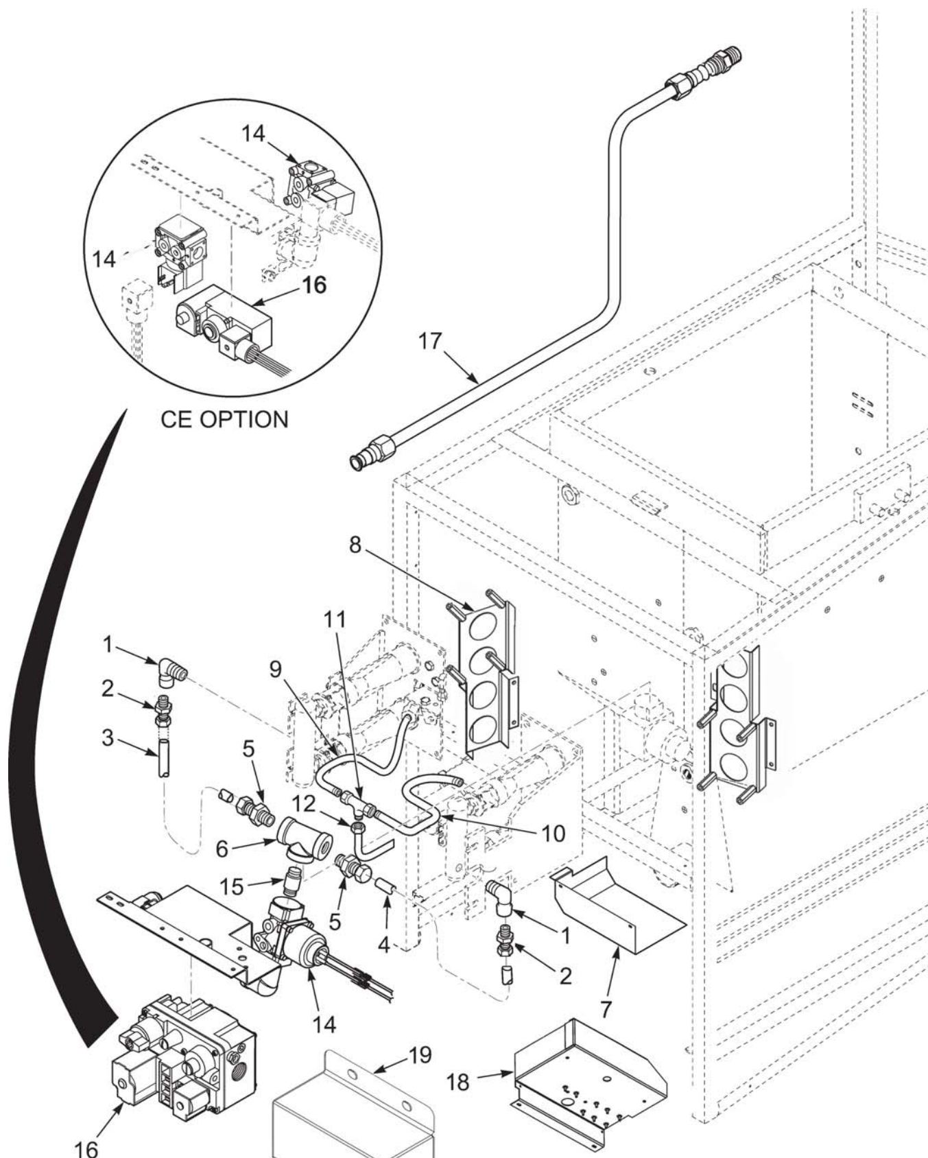
Figure 3-11. Gas Piping and Controls
