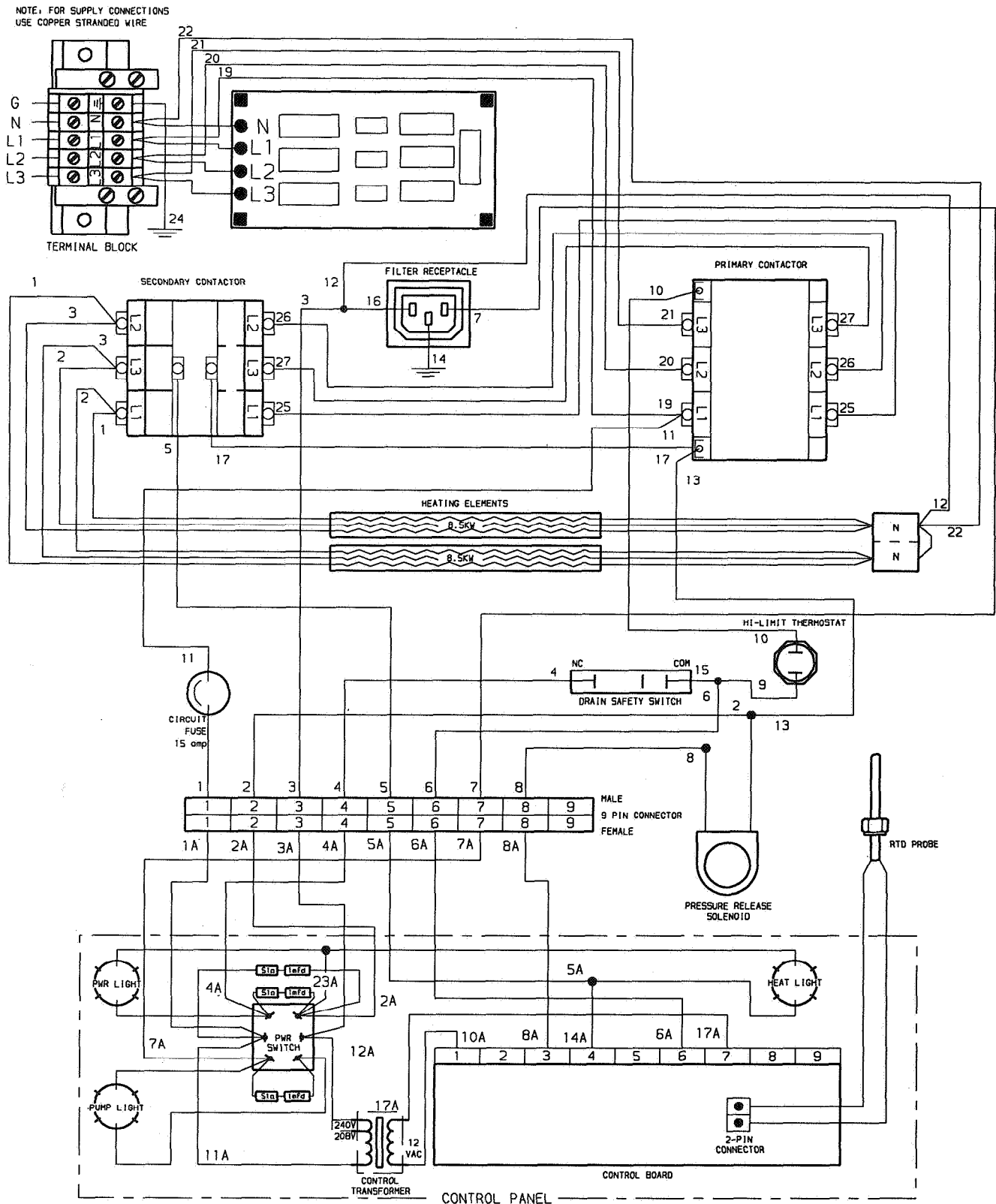
MODEL 580 ELECTRIC FRYER 400V 17KW 3N~
