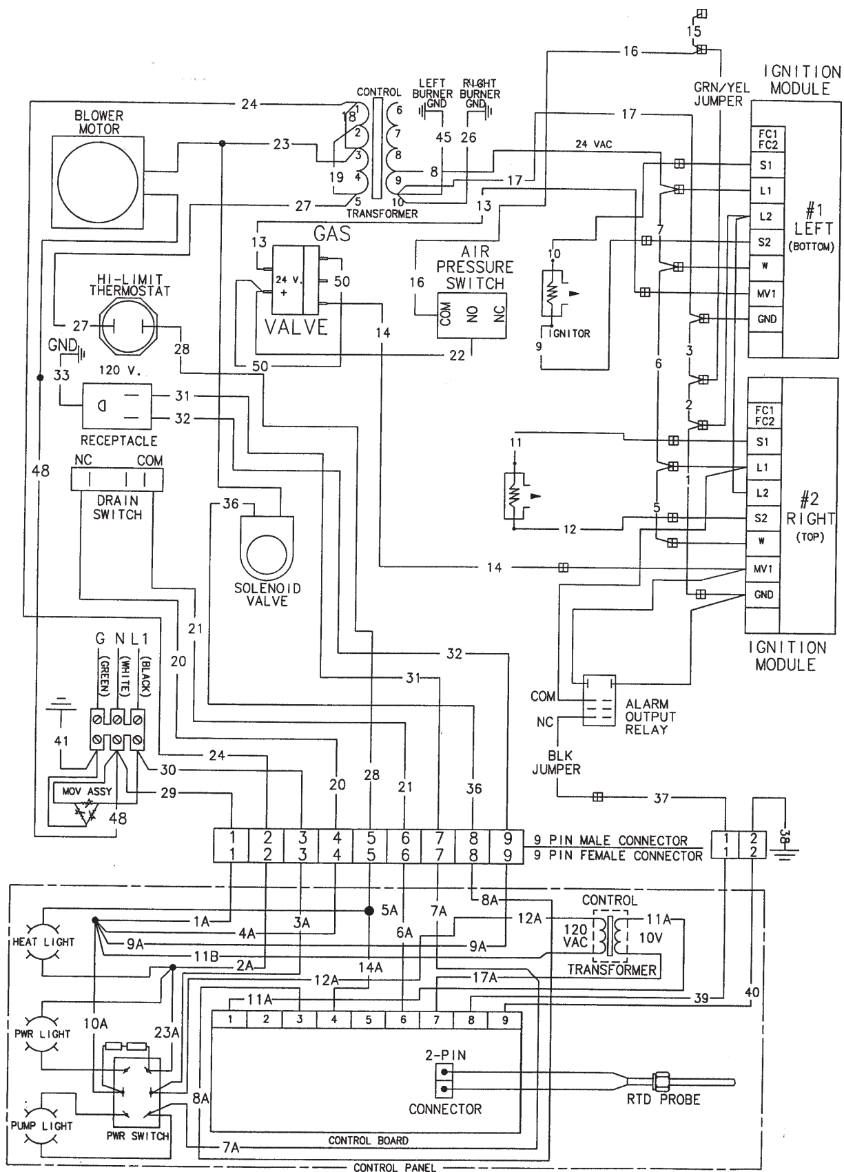
8-HEAD GAS COOKER W/LOCAL FLAME SENSING 120V 1PH 2W + G 54788
