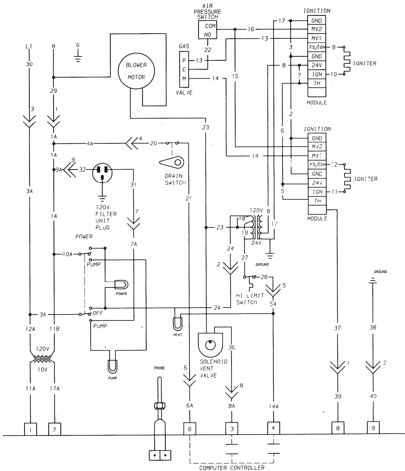
MODEL 680 GAS FRYER
