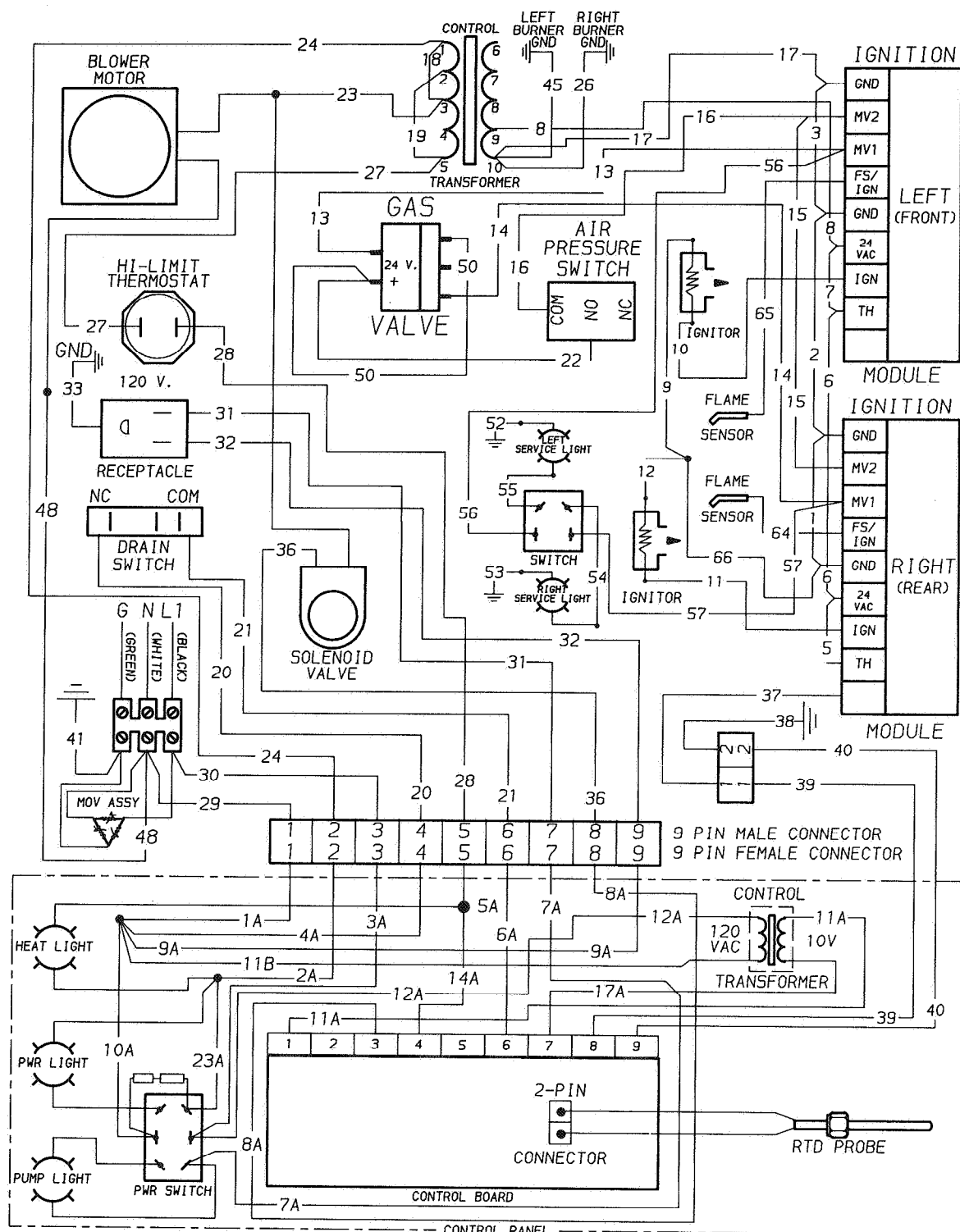
8-HEAD GAS COOKER
