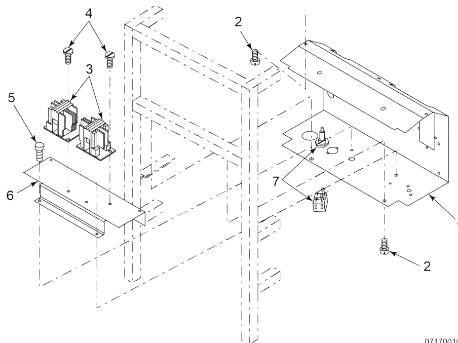
Figure 3-29 Contactor &amp; Frame Assembly (Three Phase Electric Model)
