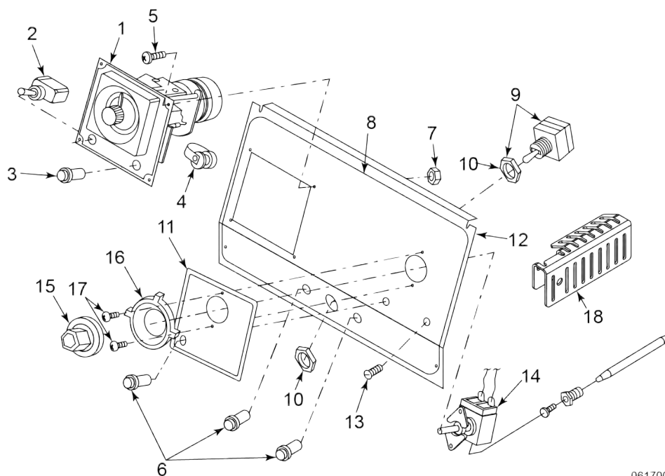
Figure 3-5 Standard Control Panel
