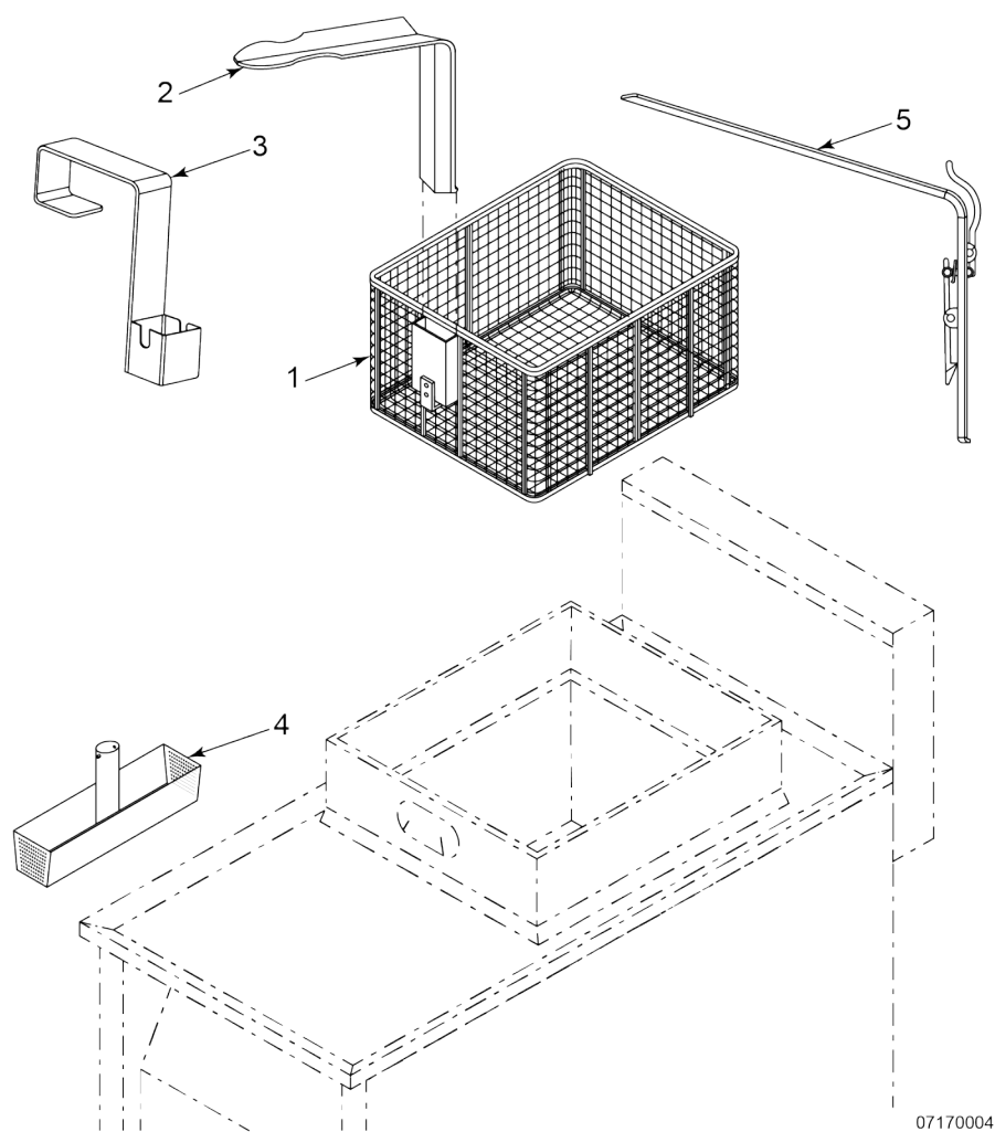
Figure 3-12 Fry Basket
