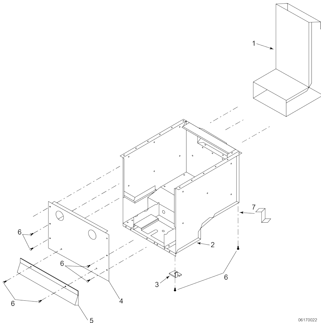
Figure 3-36 Firebox &amp; Flue Assembly (Gas Model)
