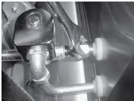
Figure 2-18 Exhaust Fitting
