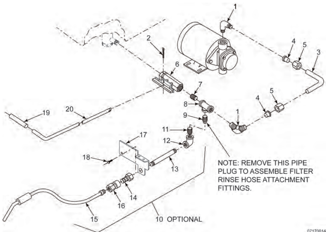
Figure 3-21 Upper Filter Plumbing Components
