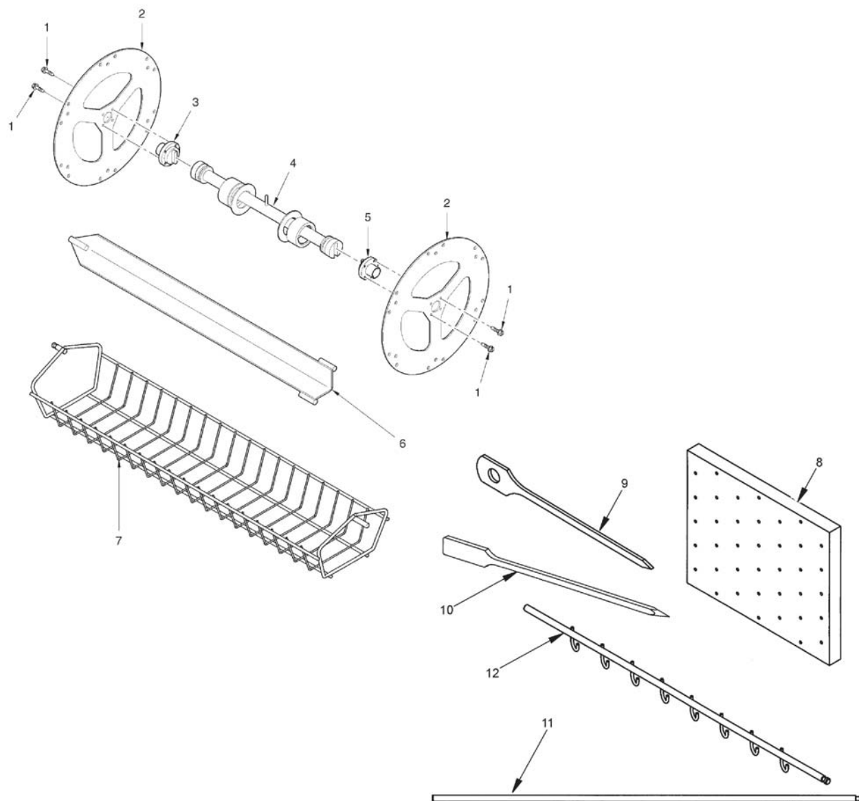
Figure 3-1. Drive Assembly
