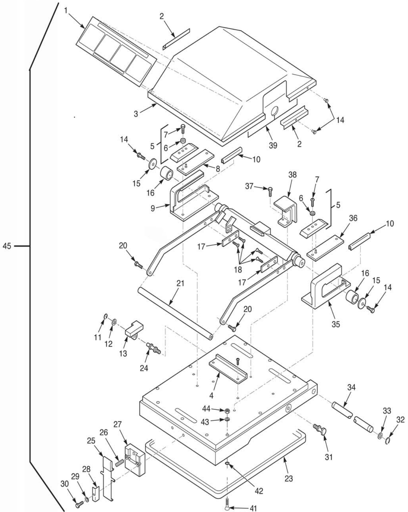
3-4. LID & COVER ASSEMBLY
