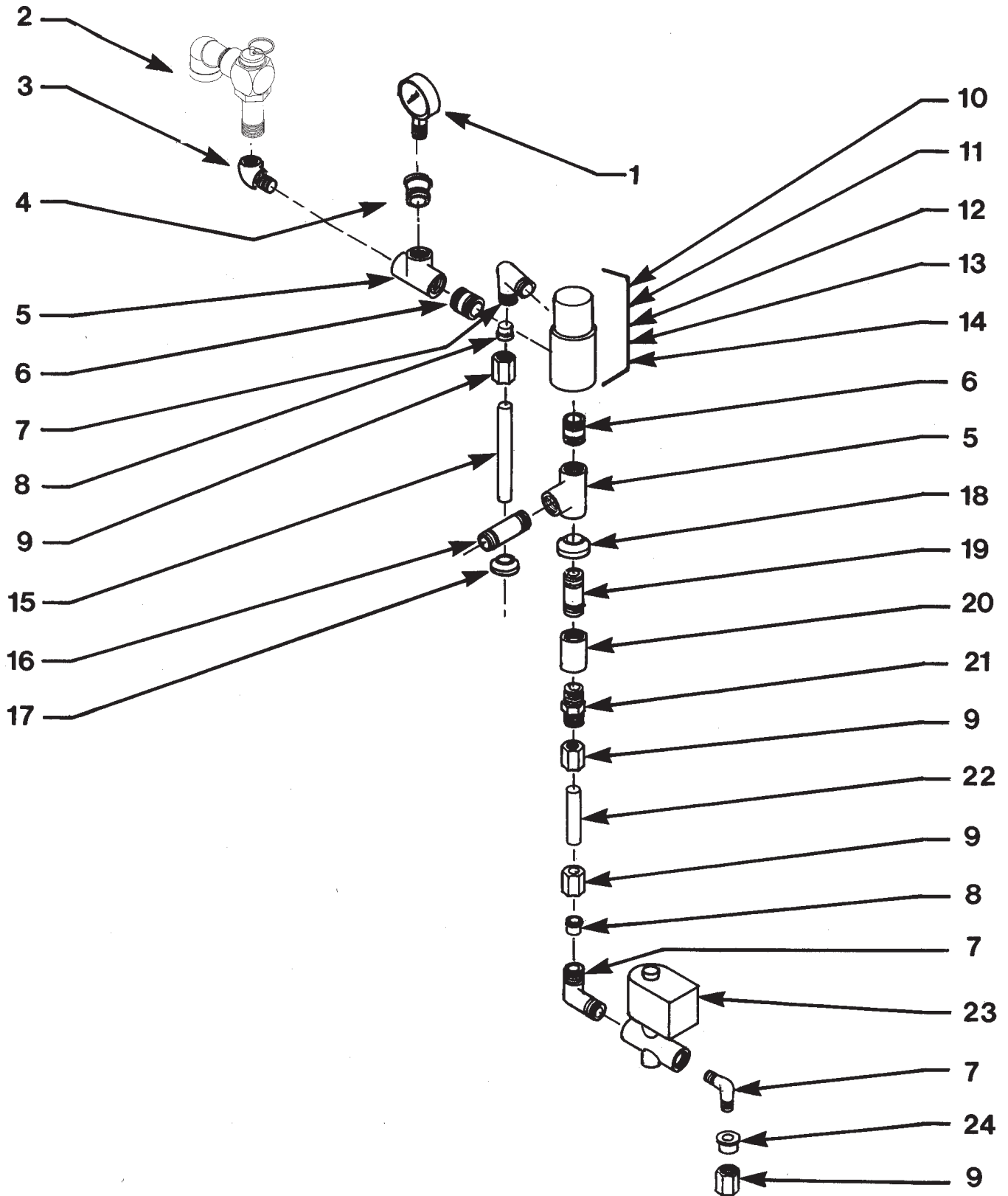
3-6. DEADWEIGHT AND SOLENOID ASSEMBLY
